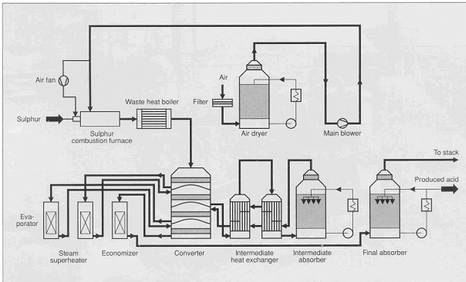
Sulphuric acid double catalysis process including sulphur combustion
